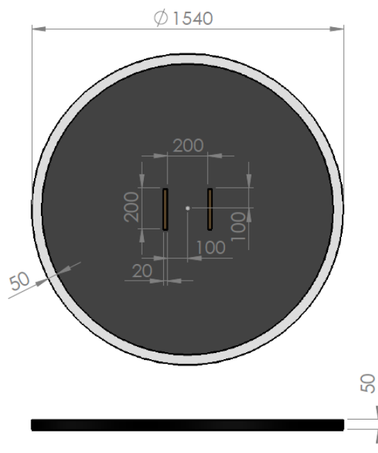
Figure 1 Dimensions of Dohyo for Sumo Robot Competition (mm)
